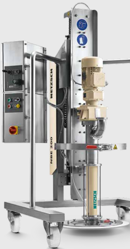
NETZSCH barrel emptying system NBE 200 with hygienic design
