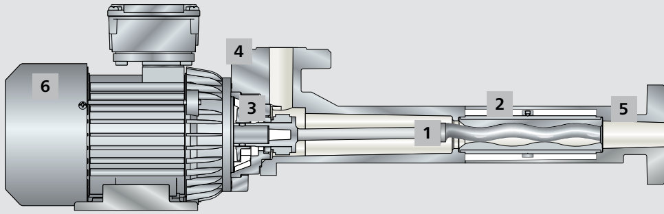
NEMO® C.Pro® Plastic Dosing Pump
