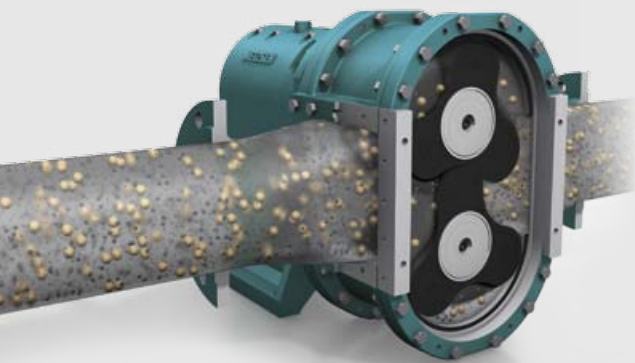
TORNADO® rotary lobe pump
