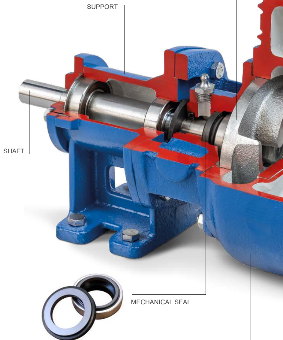
CASING
