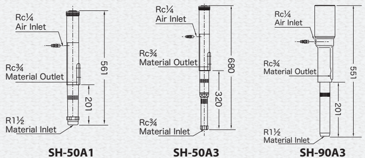
852629 SH-50A1 852634 SH-50A3 880967 SH-90A3
